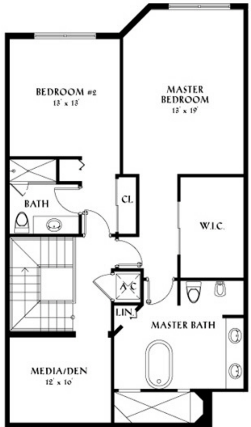
UPPER LEVEL
