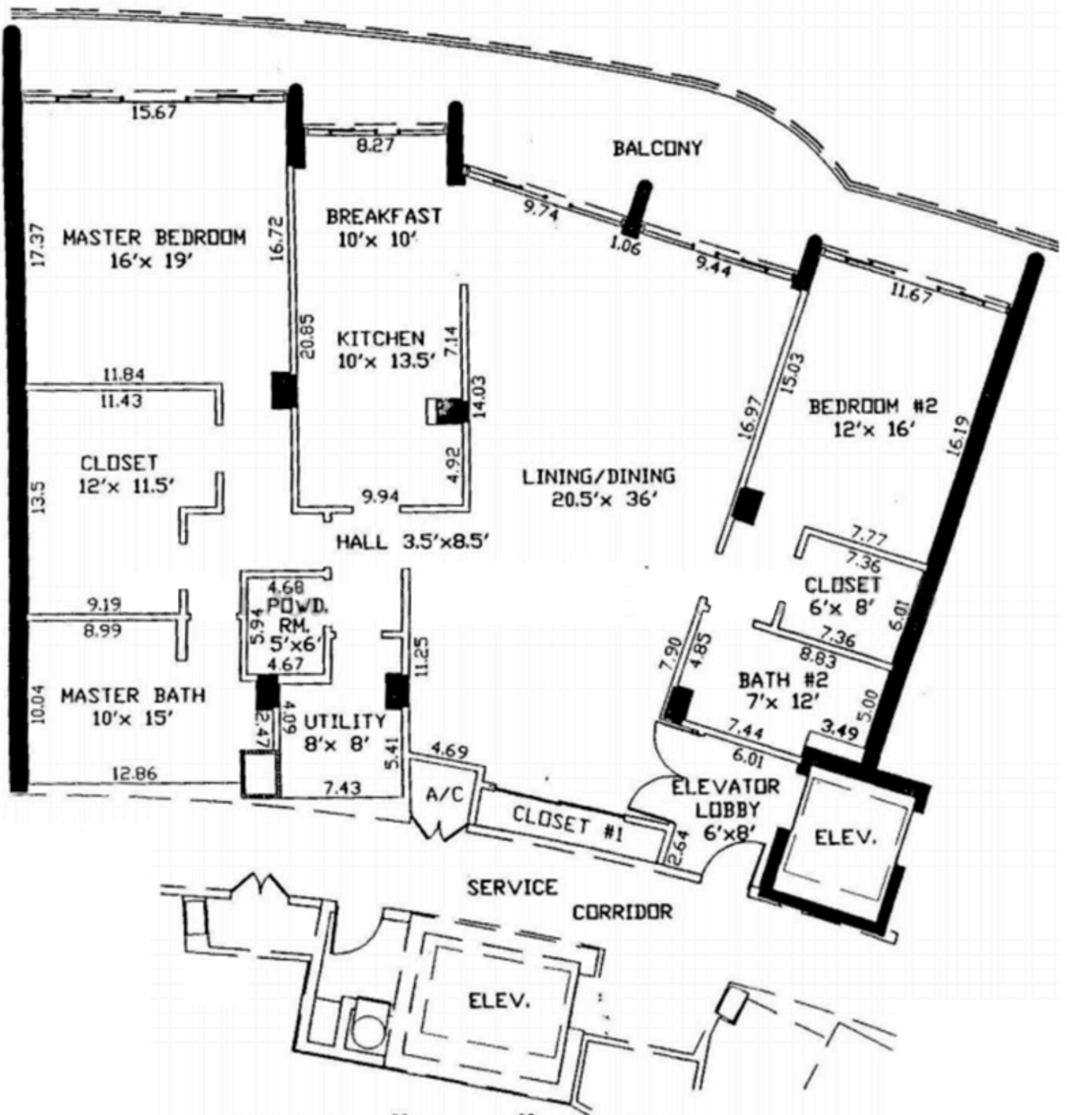
TYPE "S-4" UNIT UNIT S-404 THRU S-1704
