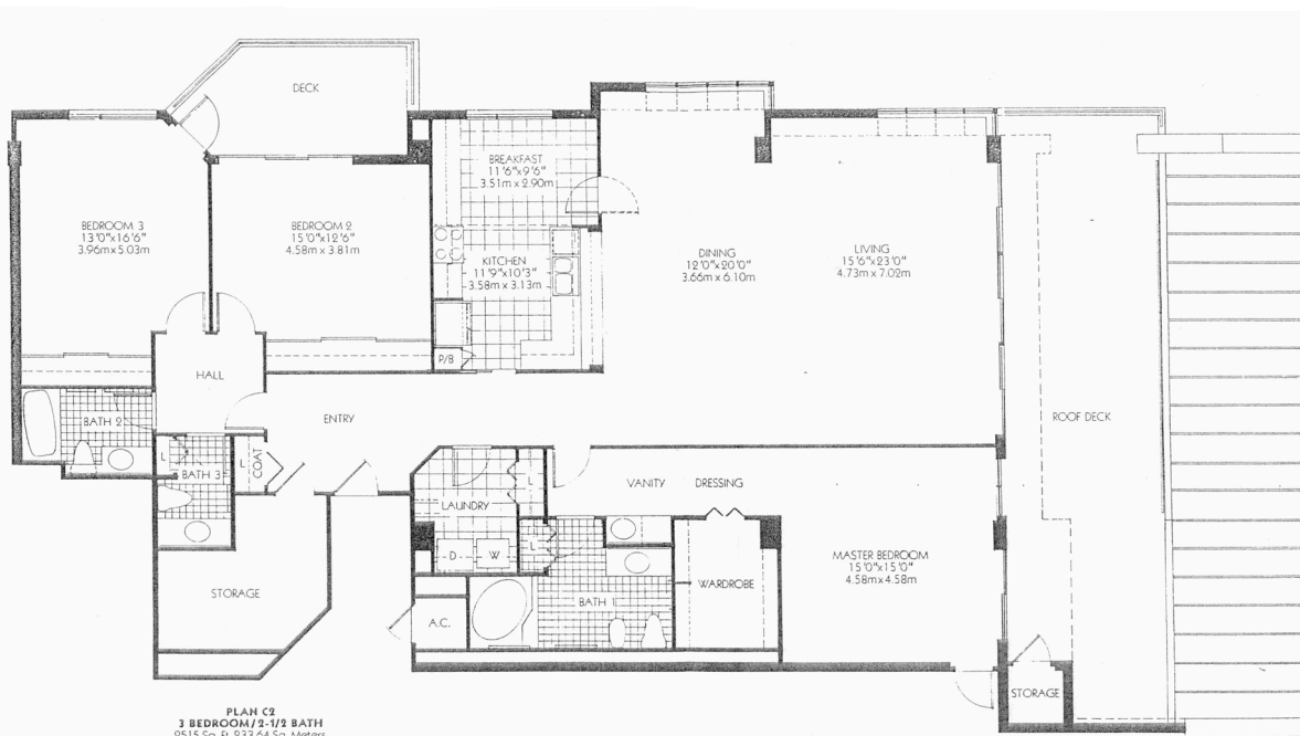
PLAN C2 3 BEDROOM / 2-1/2 BATH 9515 sq. ft. 9.33.64 Sq. Meters
