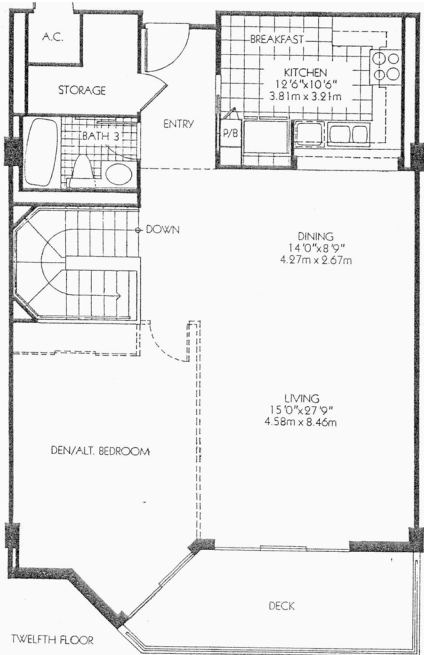
PENTHOUSE PLAN C3U 2 BEDROOM & DEN / 3 BATH (Optional 3rd Bedroom) 2176 Sq. Ft. 202.15 Sq. Meters Deck Area 307 Sq. Ft. 28.52 Sq. Meters
