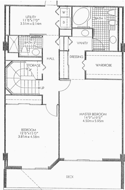
PENTHOUSE PLAN C3U 2 BEDROOM & DEN / 3 BATH (Optional 3rd Bedroom) 2176 Sq. Ft. 202.15 Sq. Meters Deck Area 307 Sq. Ft. 28.52 Sq. Meters
