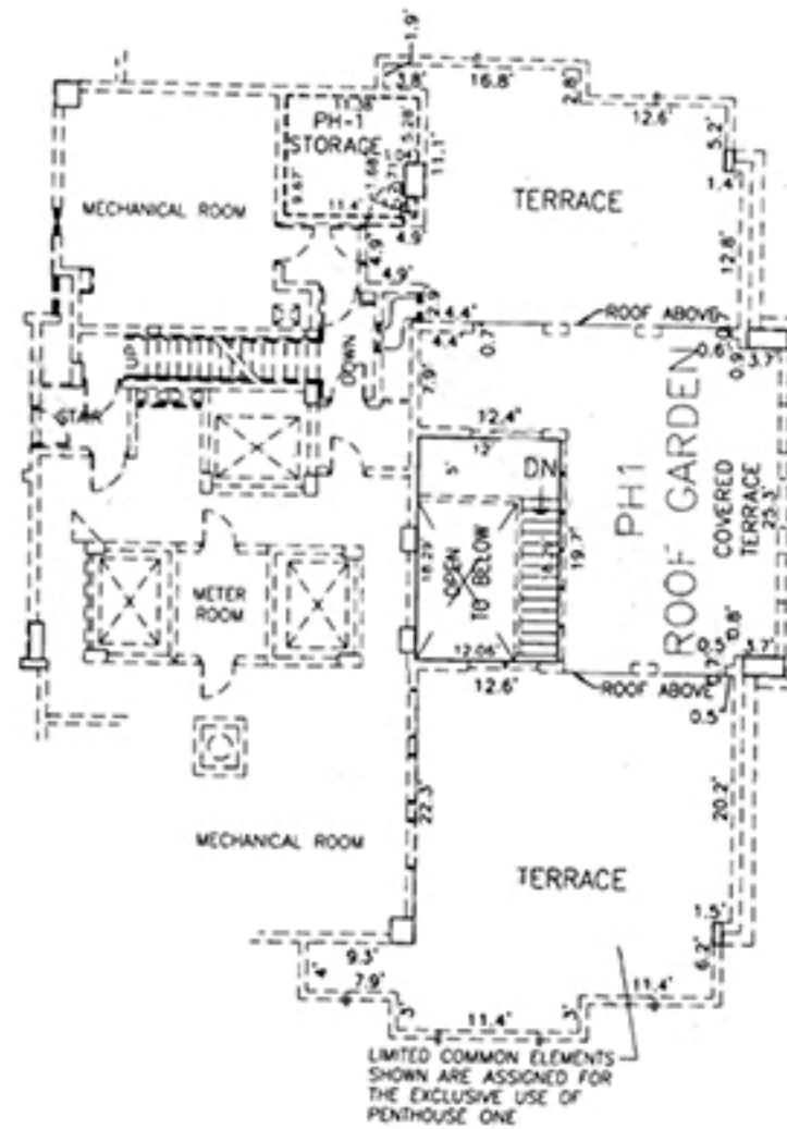
ROOF LEVEL
