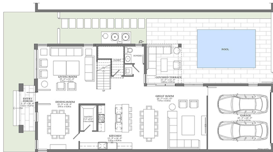
FIRST LEVEL 1,600 A/C SF » 148.64 M 2
