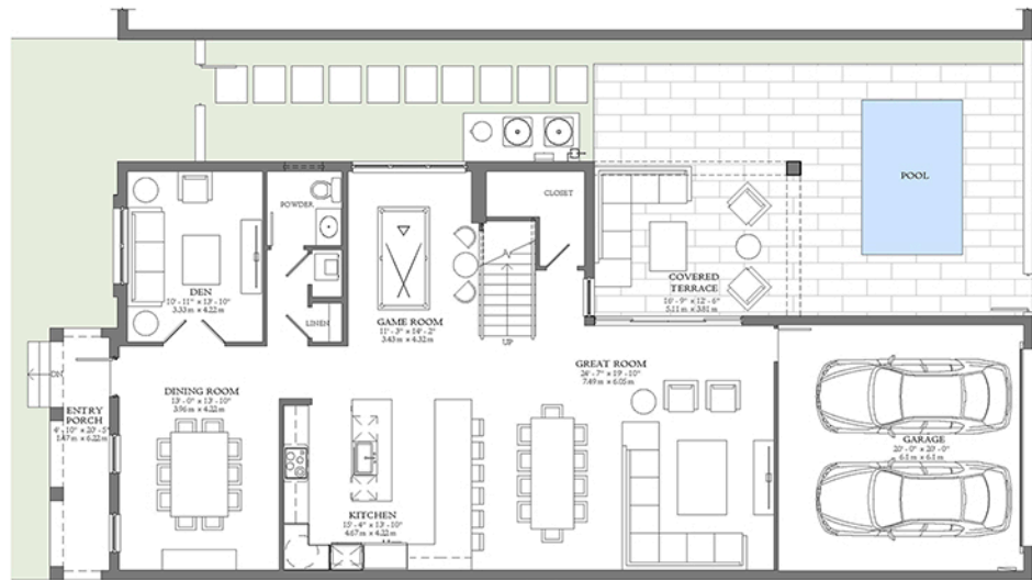
FIRST LEVEL 1,642 A/C SF » 152.53 M 2
