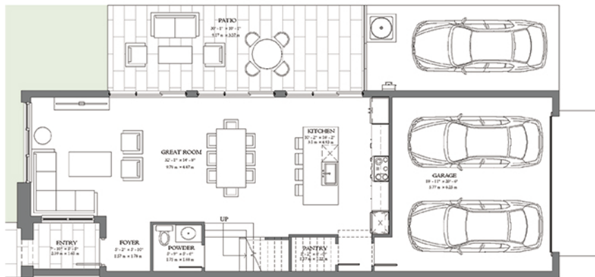
GROUND LEVEL 890 A/C SF » 82.68 M 2
