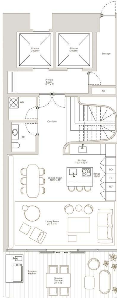
FIRST FLOOR
