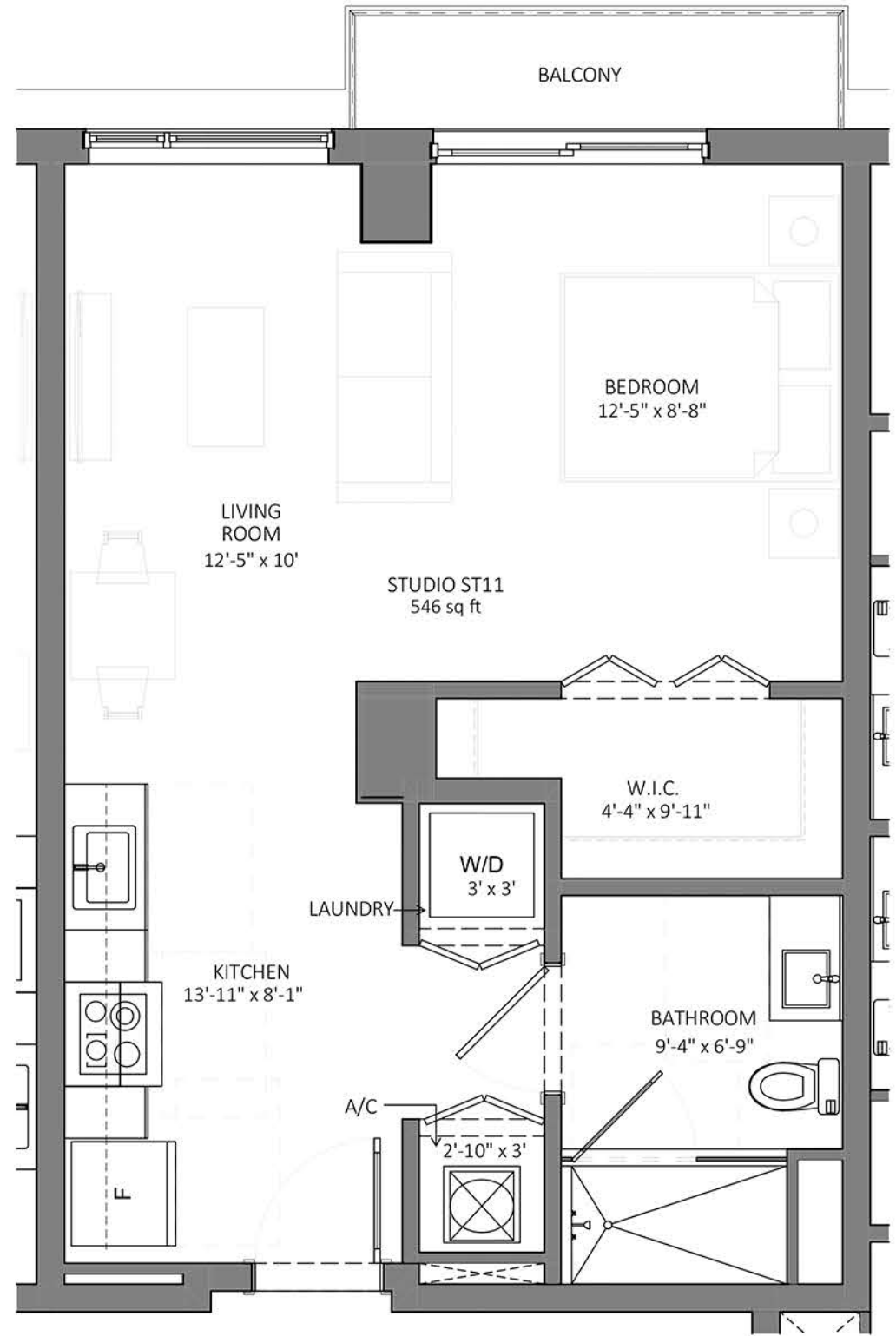
ST11 STUDIO UNIT ST11 SCALE: 1/4" = 1'-0"
